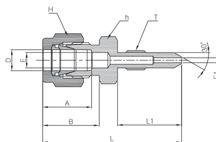
1U thread calibration fitting for Honeywell DP transmitters
