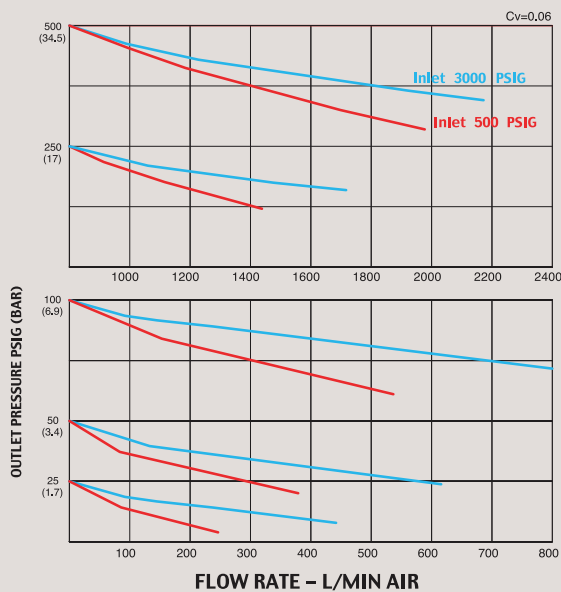
REGULATOR DISCHARGE CHARACTERISTICS CURVES
